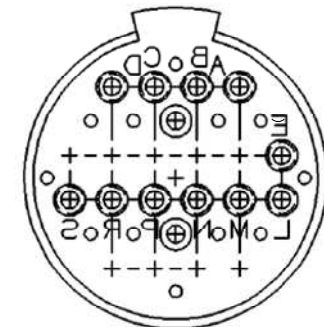
Pin Location
